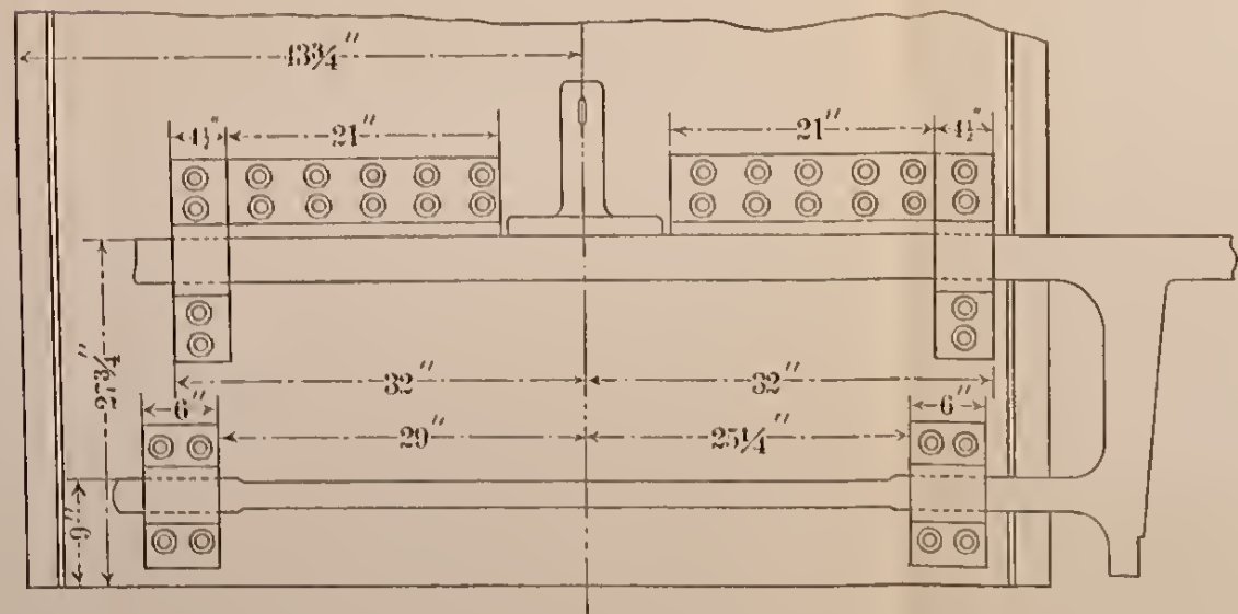
FIG. 4 EXPANSION PADS
